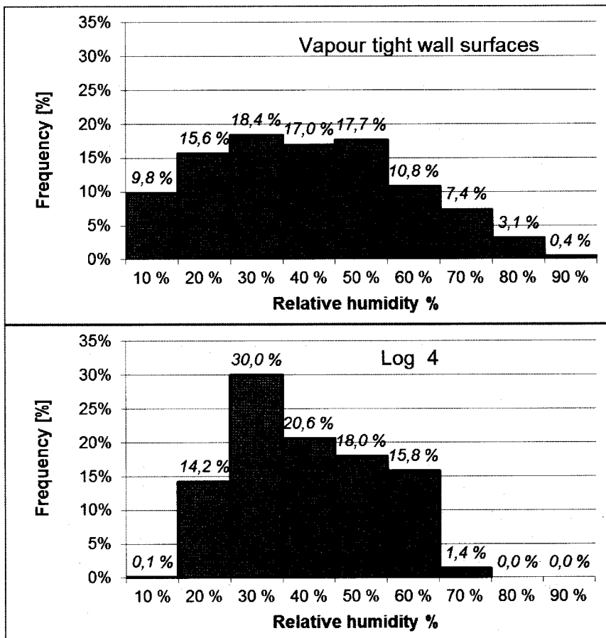
Figure 5 : Incidence of different relative humidity areas during one year in Vapor tight –case (above) and Log 4 –case (below).
