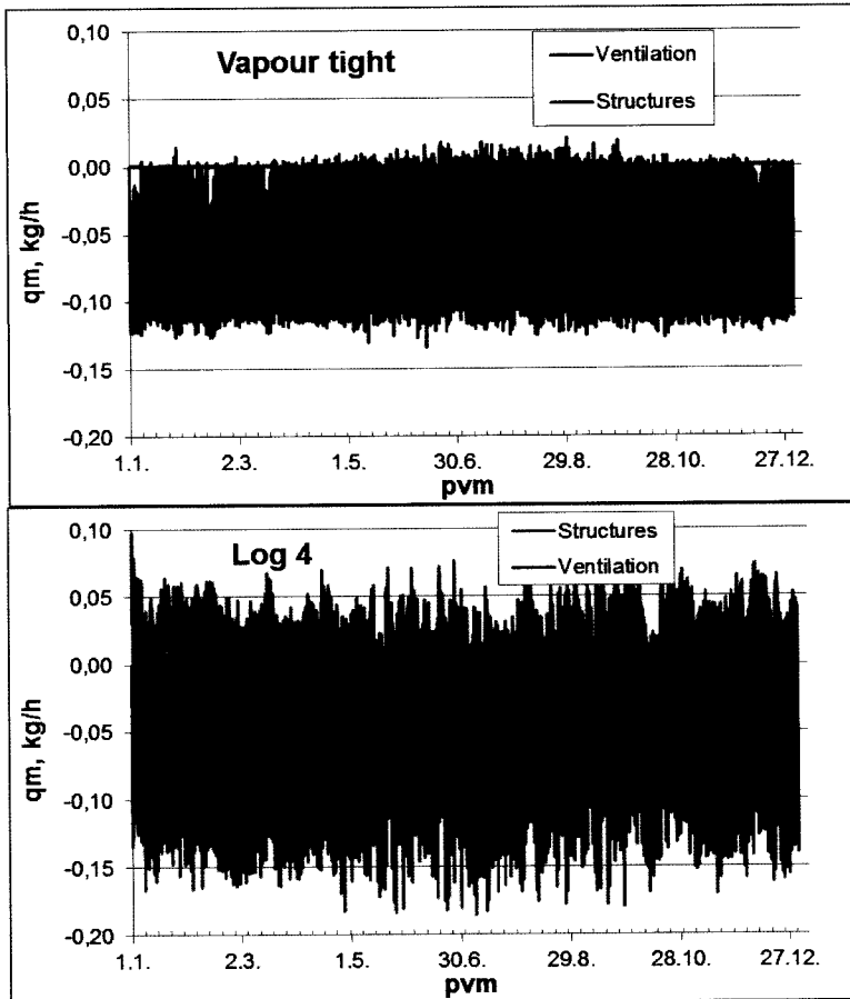
Figure 2 : Moisture flow rates between indoor air and structures and that caused by ventilation. Cases having vapor tight structure surfaces (above) and four log walls (below). Negative value means that moisture is removed from indoor air.
