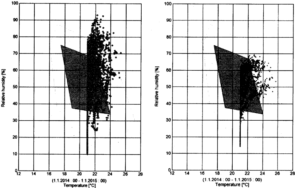
Figure 4 : The hourly solved indoor temperature and relative humidity conditions and comparison to comfort conditions. Case Vapour tight is on the left side and Log 4 on the right side. Green area corresponds to comfortable conditions and the light yellow to 'still comfortable' conditions [5].
